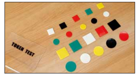
Obr. 1. Token test.
